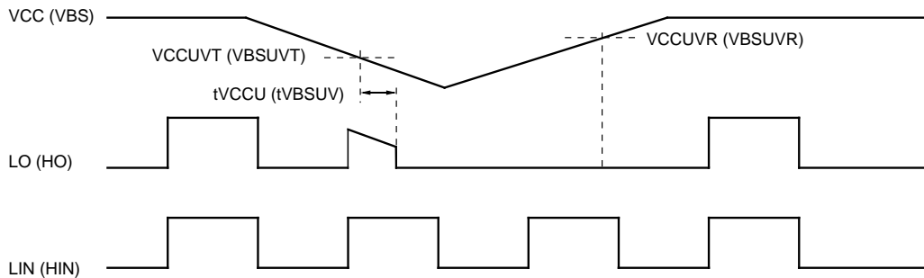
2. VCC(VBS) Supply Undervoltage Lockout Timing Diagram
