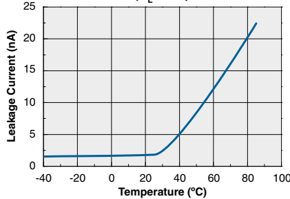
CPC1335 TVS Diode Leakage vs. Temperature (Pins 7 & 8) ( V_L=40V )
