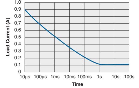
CPC1335 Energy Rating Curve
