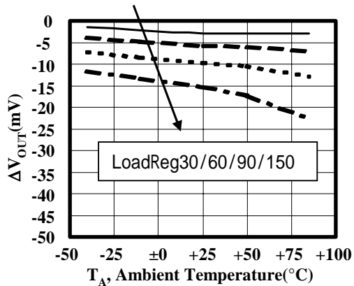
■ \Delta V_{OUT} versus Ambient Temperature of the TK11130CS
