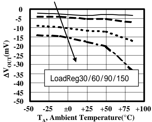
■ \Delta V_{OUT} versus Ambient Temperature of the TK11140CS
