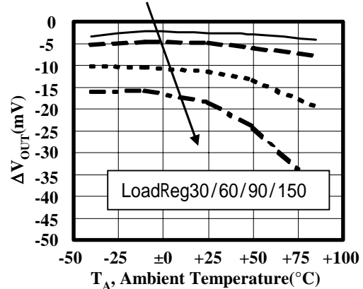
■ \Delta V_{OUT} versus Ambient Temperature of the TK11150CS
