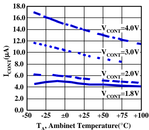
■ Control Current versus Ambient Temperature
