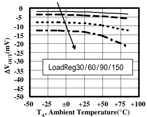
■ \Delta V_{OUT} versus Ambient Temperature of the TK11120CS
