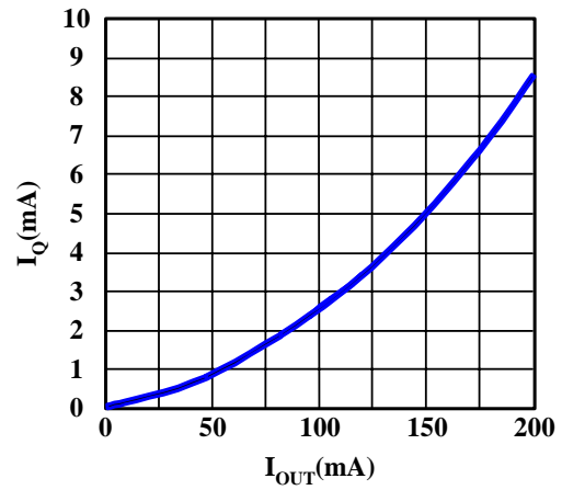
■ Quiescent Current versus Output Current
