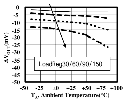
■ \Delta V_{OUT} versus Ambient Temperature of the TK11133CS
