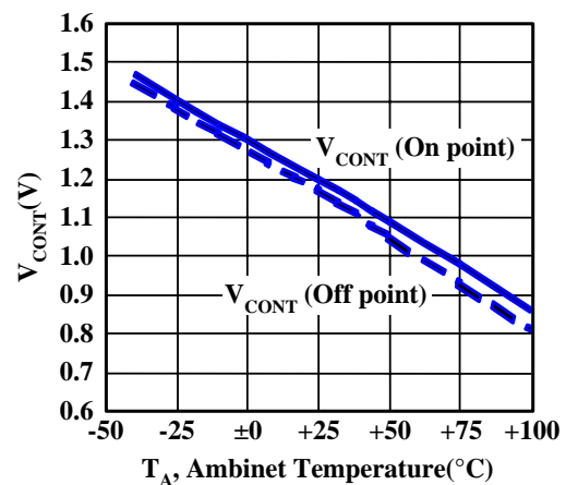
■ Control Voltage versus Ambient Temperature
