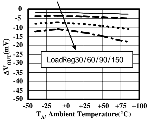
■ \Delta V_{OUT} versus Ambient Temperature of the TK1115CS
