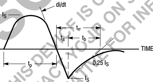
Figure 15. Diode Reverse Recovery Waveform
