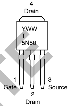
CASE 369 DPAK (Straight Lead) STYLE 2
