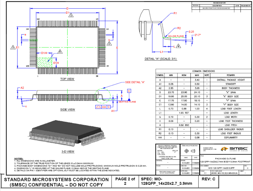
Figure 2 128-Pin QFP Package Outline (3.9mm footprint)
