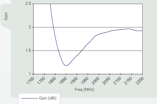
Radiating Element Average Gain
