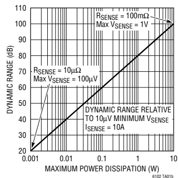
Dynamic Range vs Maximum Power Dissipation in R_{\text{SENSE}} at 10A
