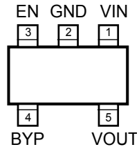
MIC5319-x.xBD5/YD5 TSOT-23-5 (D5) (Top View)
