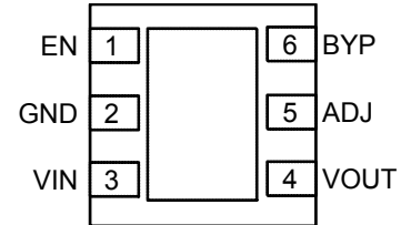
MIC5319BML/YML (Adjustable) 6-Pin 2mm x 2mm MLF™ (ML) (Top View)
