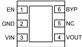
MIC5319-x.xBML/YML 6-Pin 2mm x 2mm MLF™ (ML) (Top View)
