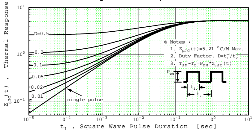
Fig 11. Thermal Response
