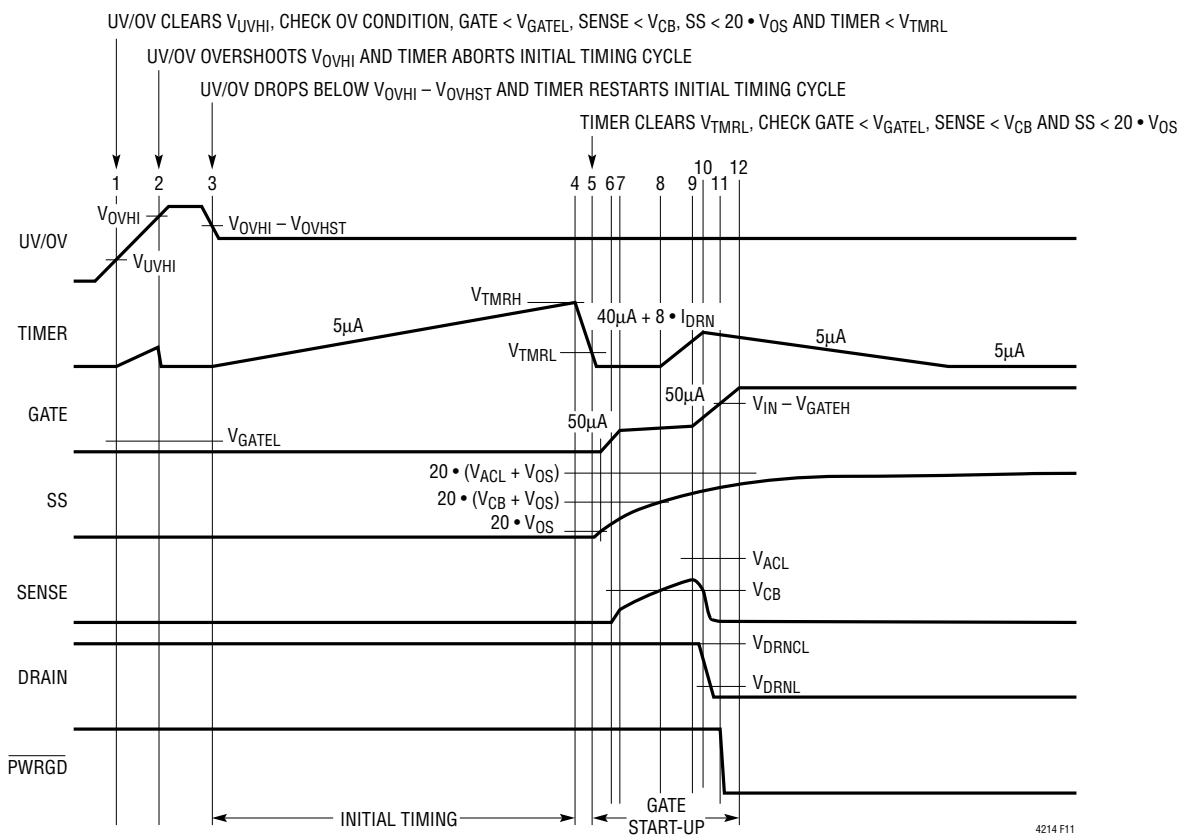
Figure 11. Undervoltage Timing with an Overtoltage Glitch (All Waveforms are Referenced to V EE )
