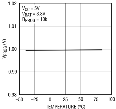
PROG Pin Voltage vs Temperature (Constant-Current Mode)
