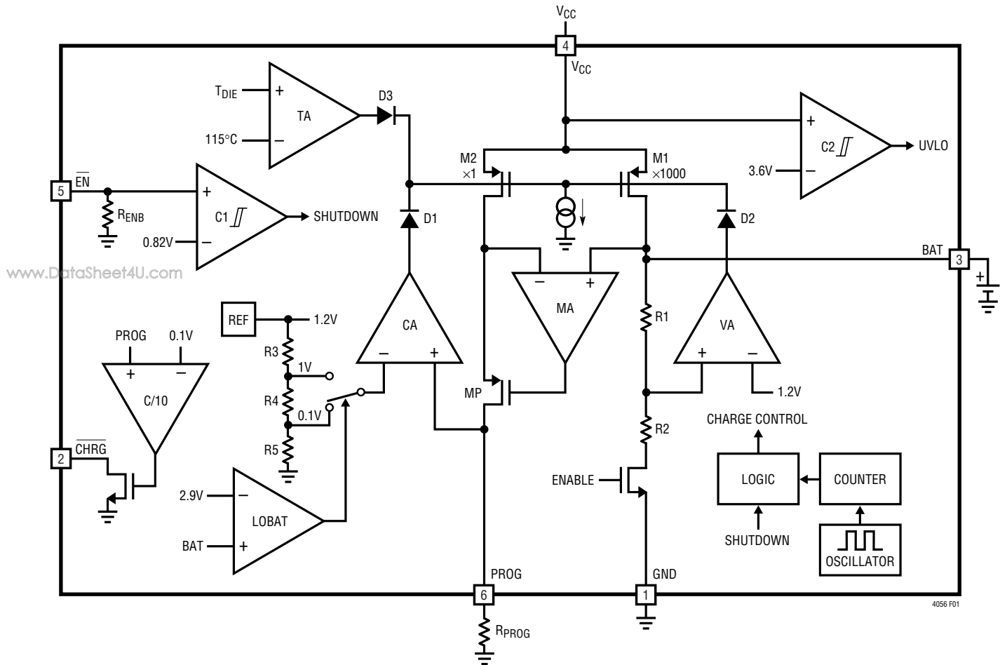
Figure 1. LTC4065-4.4 Block Diagram
