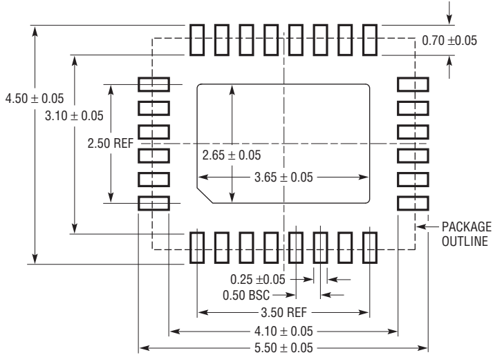
UFD Package 28-Lead Plastic QFN (4mm × 5mm) (Reference LTC DWG # 05-08-1712 Rev B)
