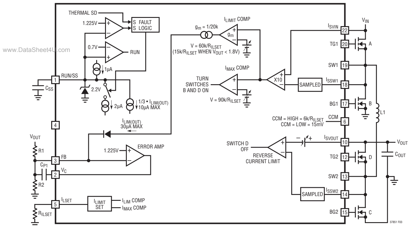
Figure 3. Block Diagram of Current Limit Fault Circuitry
