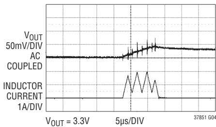
Burst Mode Ripple
