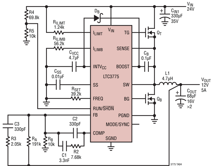
24V Input, 12V/5A Output at 500kHz
