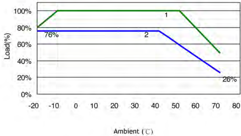
Open-Frame (PMK130T-xx) :
