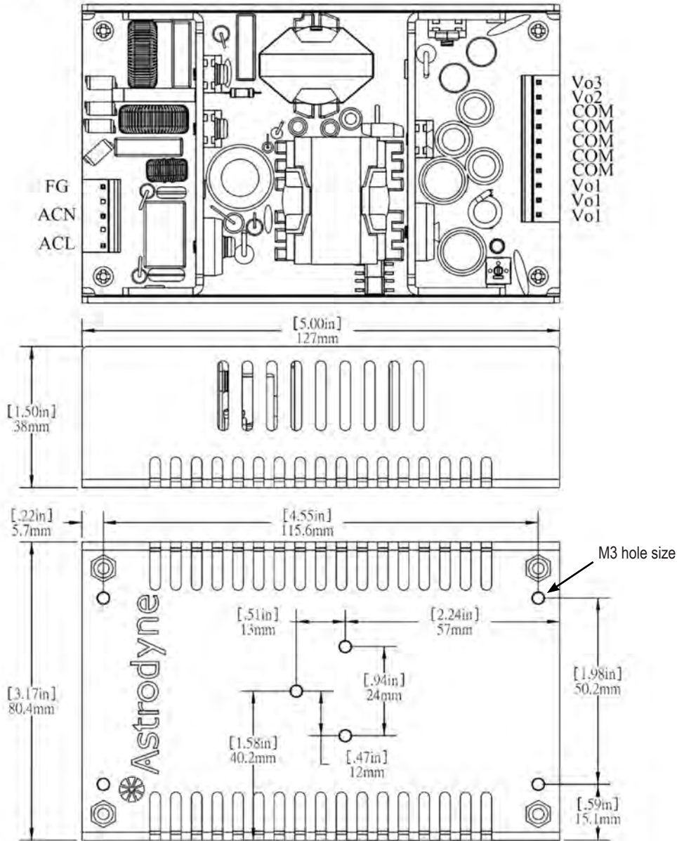
U-Bracket (PMK130T-xxU-A) :
