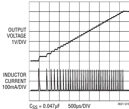
Soft-Start Waveforms
