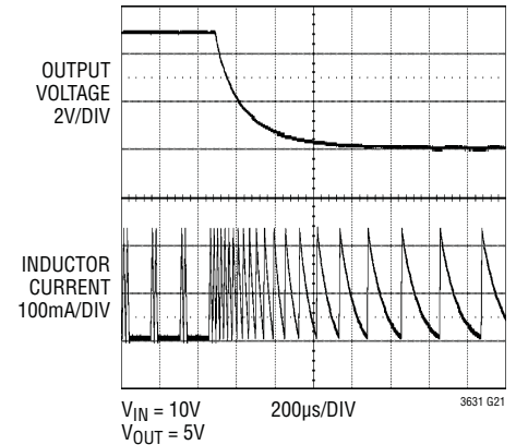
Short-Circuit Response
