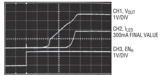
Start-Up Transient
