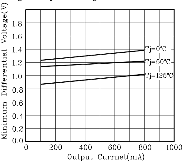
Fig. 5 Dropout Voltage
