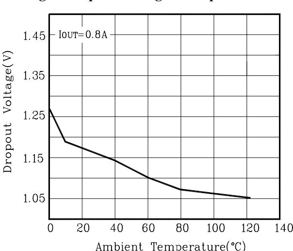
Fig. 6 Dropout Voltage - Temperature
