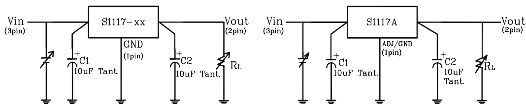
Fig. 1 Fixed Voltage Regulator
