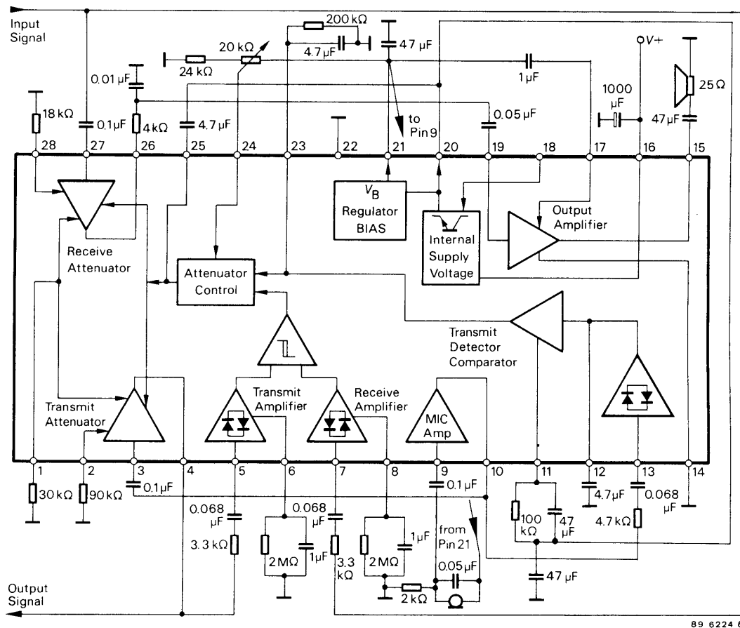
Figure 1. Block diagram and application circuit
