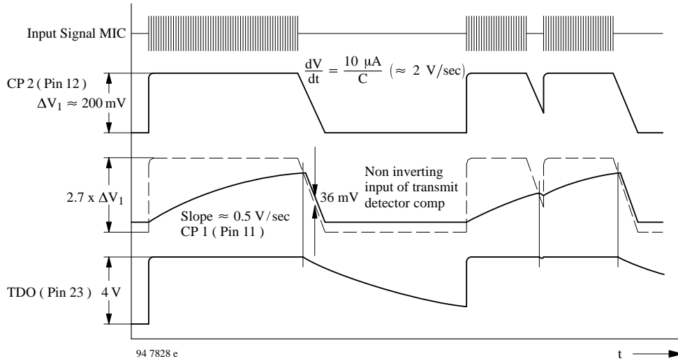
Figure 11. Transmit detector operation
