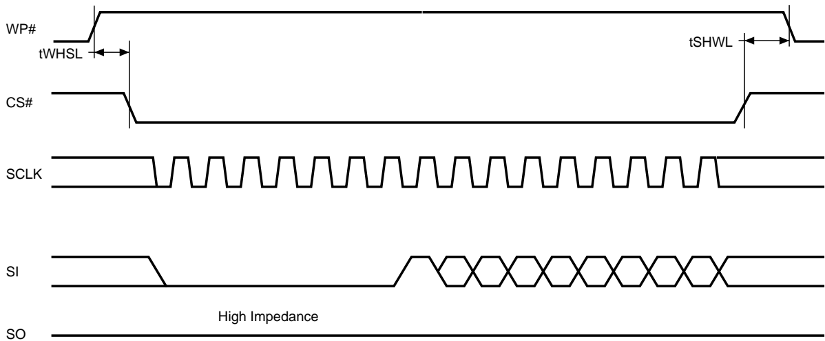
Figure 8. Write Protect Setup and Hold Timing during WRSR when SRWD=1
