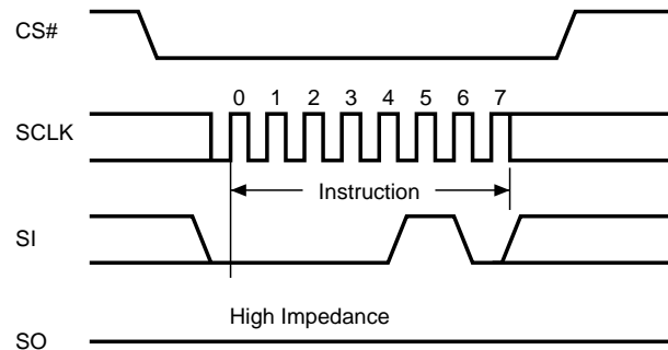
Figure 11. Write Enable (WREN) Instruction Sequence
