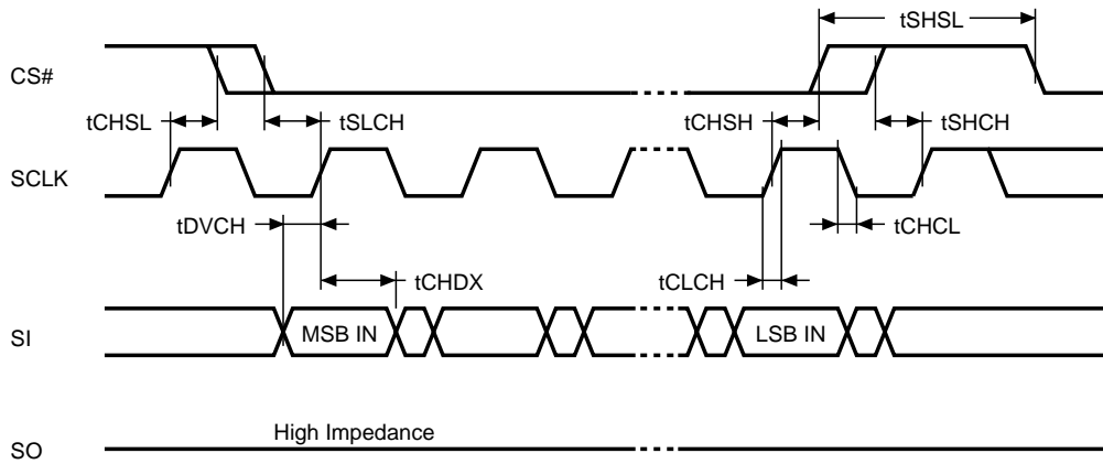
Figure 7. Serial Input Timing
