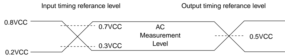
Figure 5. INPUT TEST WAVEFORMS AND MEASUREMENT LEVEL
