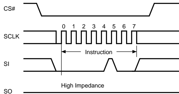
Figure 12. Write Disable (WRDI) Instruction Sequence
