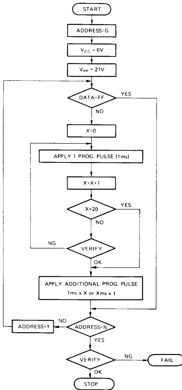
Fig. 17—PROGRAMMING FLOW CHART FOR Quick Pro™
