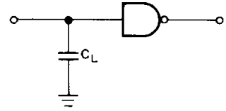
Fig.2 – AC TEST CONDITIONS (INCLUDING PROGRAMMING)
