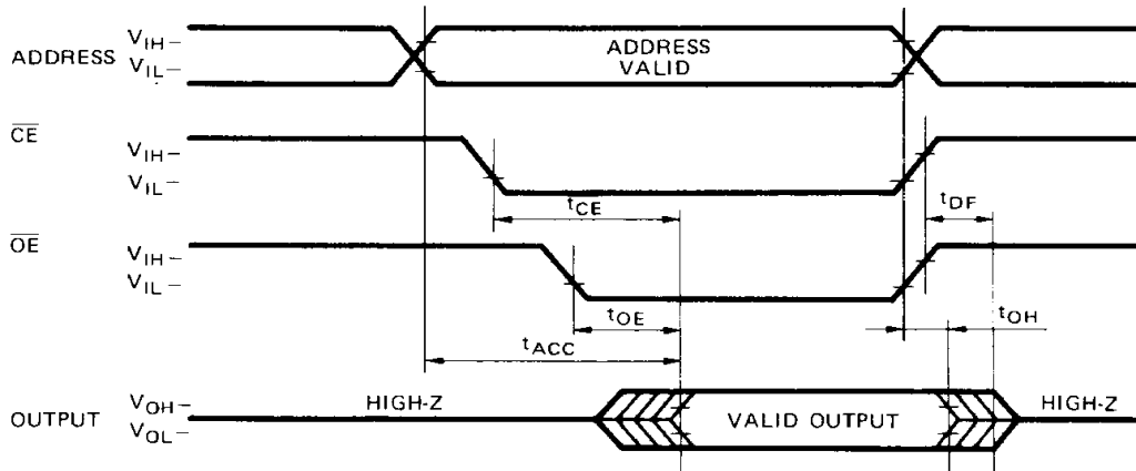
OPERATION TIMING DIAGRAM
