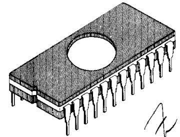
CERDIP PACKAGE DIP-24C-C02
