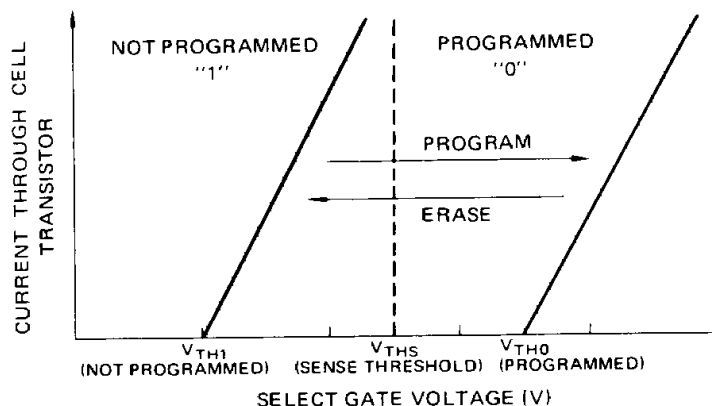
Fig. 15 — MEMORY CELL THRESHOLD SHIFT
