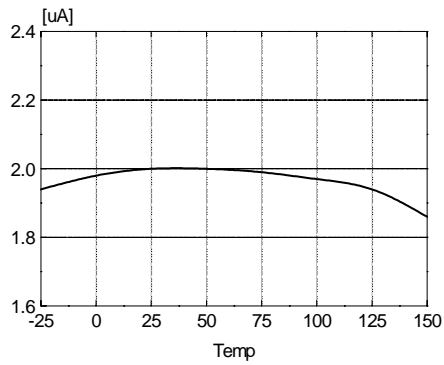
Figure 9. Shutdown Delay Current vs. Temp.
