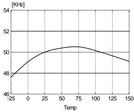
Figure 15. Burst Mode Frequency vs. Temp.
