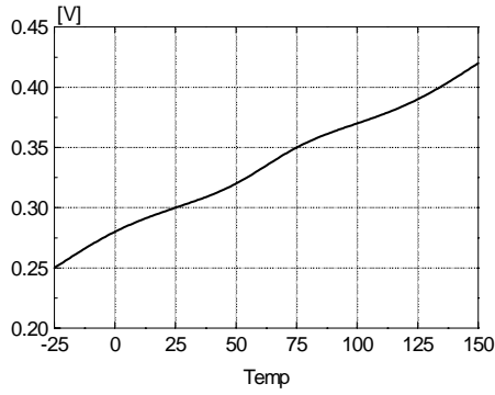
Figure 7. Feedback Offset Voltage vs. Temp.
