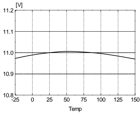
Figure 13. Burst Mode Low Voltage vs. Temp.
