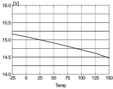
Figure 3. Start Threshold Voltage vs. Temp.
