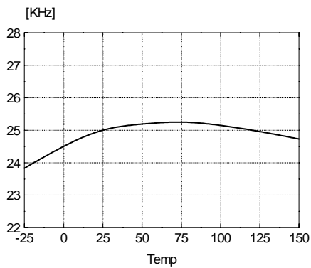
Figure 5. Initial Frequency vs. Temp.
