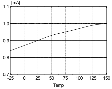
Figure 8. Feedback Source Current vs. Temp.
