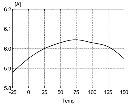
Figure 18. Over Current Limit vs. Temp.
