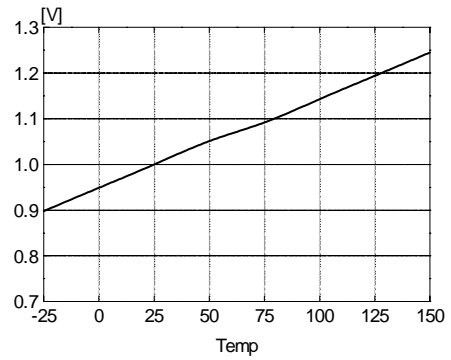
Figure 16. Burst Mode Enable Voltage vs. Temp.
