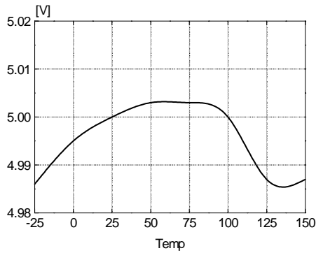
Figure 11. Softstart Voltage vs. Temp.
