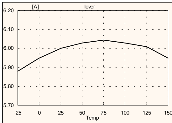
Figure 18. Peak Current Limit vs. Temp.
