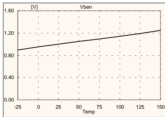
Figure 16. Burst Mode Enable Voltage vs. Temp.
