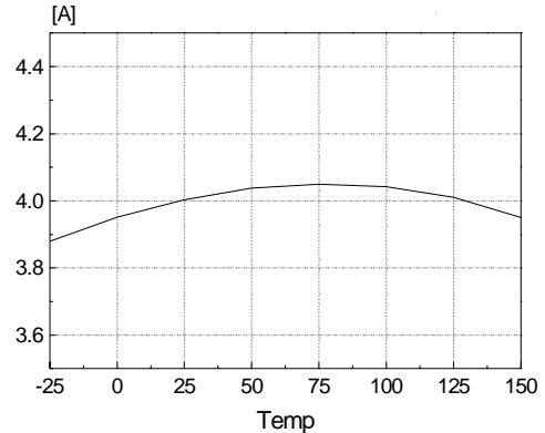
Figure 18. Peak Current Limit vs. Temp.
