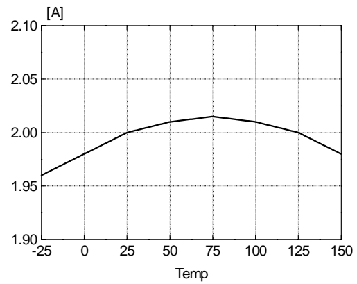
Figure 16. Over Current Limit vs. Temp
