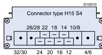
H15 S4 connectors for 20 and 25 A types
