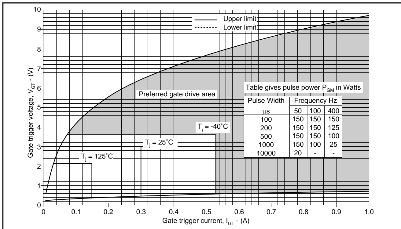
Fig.4 Gate characteristics
