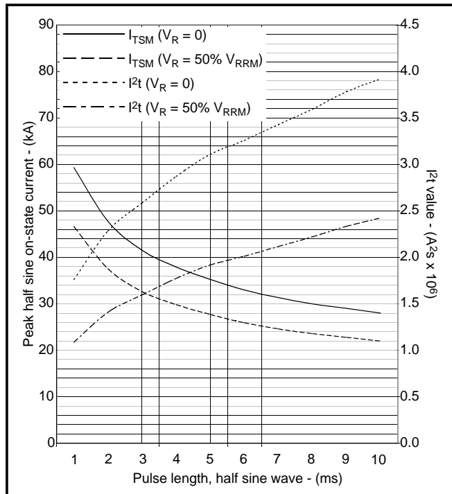
Fig.8 Sub-cycle surge currents
