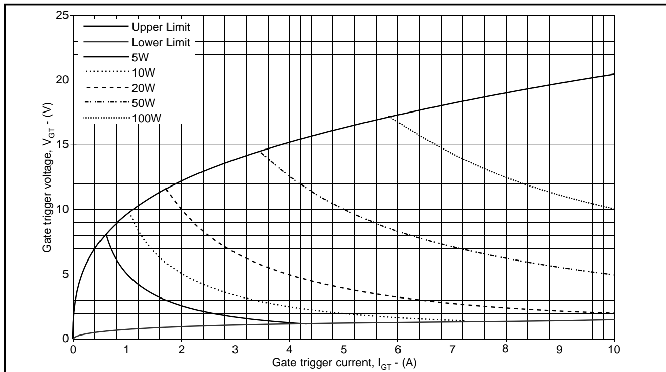
Fig.5 Gate characteristics
