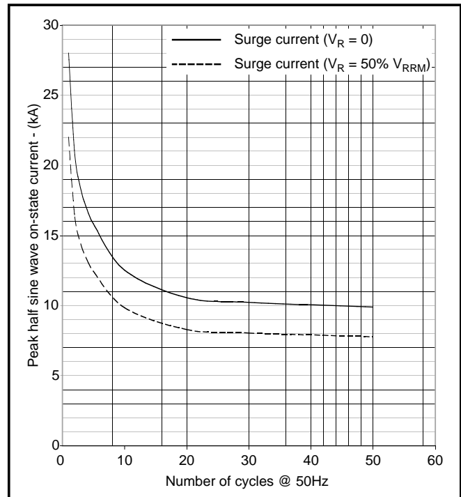
Fig.9 Multi-cycle surge currents
