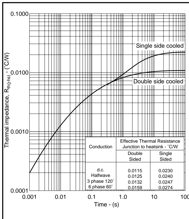
Fig.6 Transient thermal impedance - junction to heatsink
