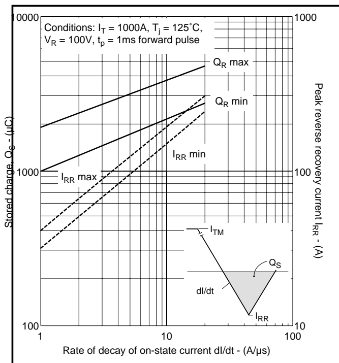
Fig.4 Stored charge
