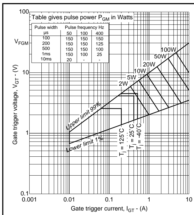
Fig.5 Gate characteristics
