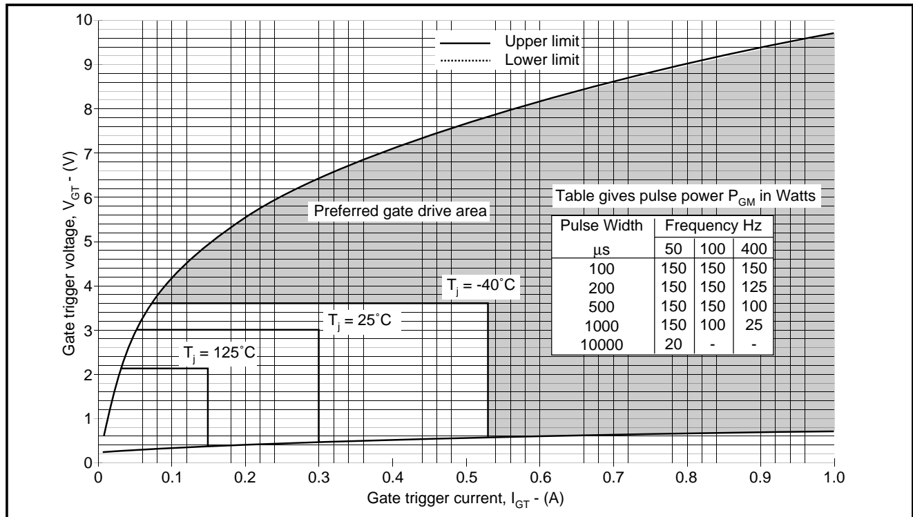
Fig.8 Gate characteristics
