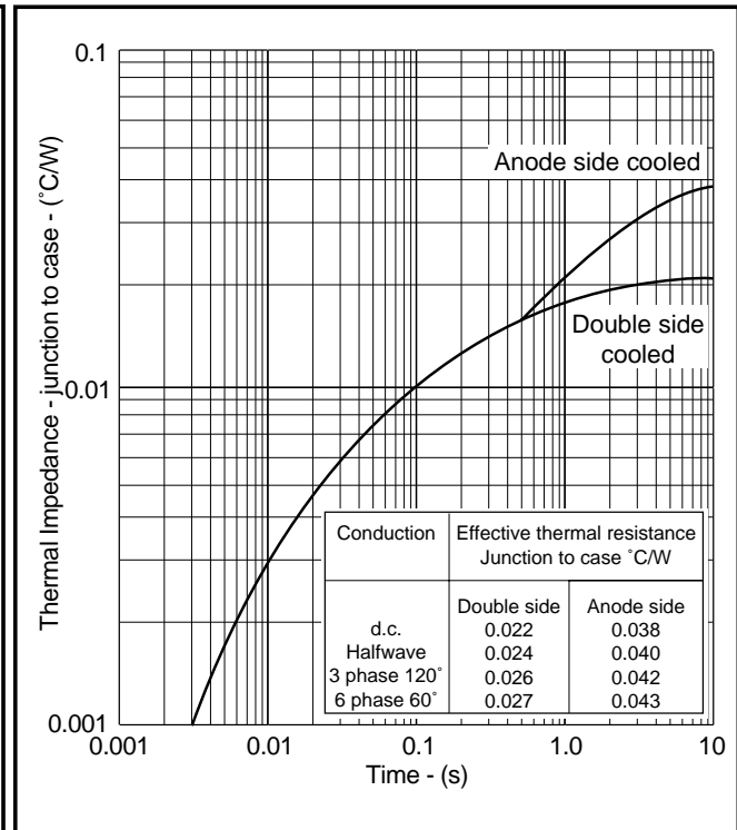
Fig.13 Transient thermal impedance - junction to case
