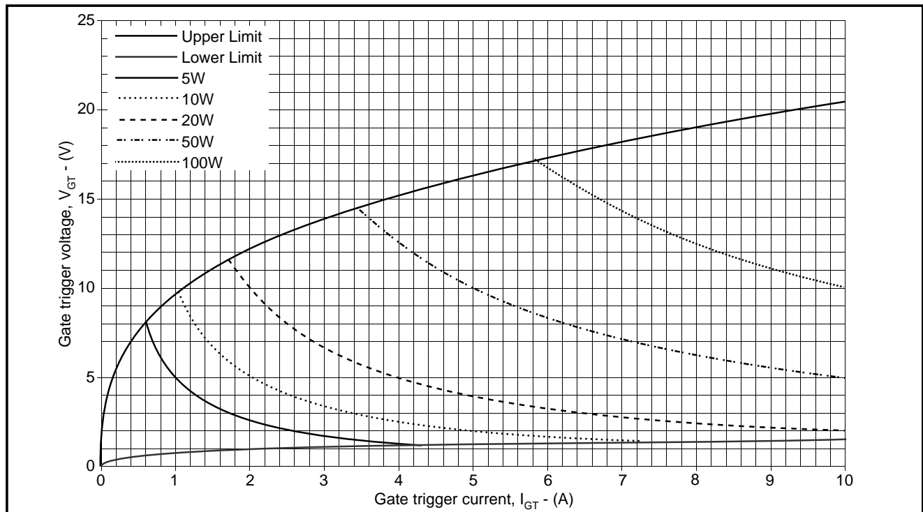
Fig.9 Gate characteristics
