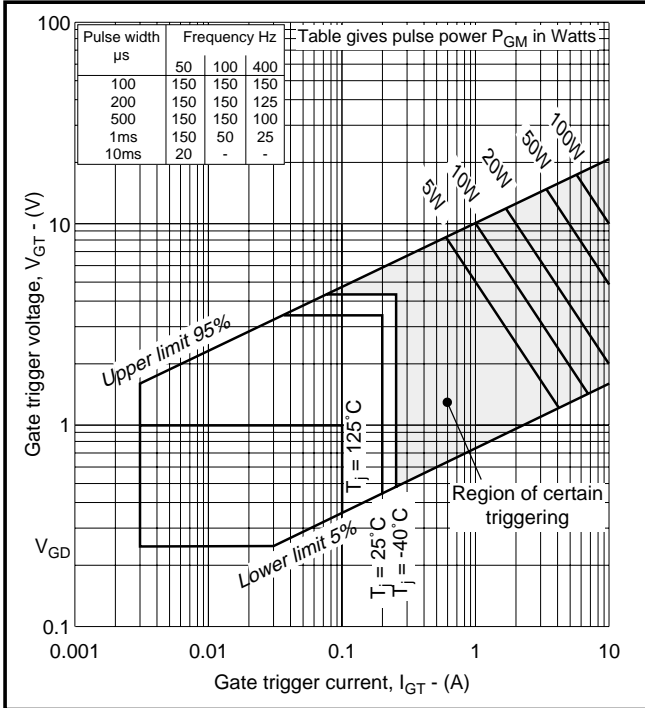
Fig.6 Gate characteristics
