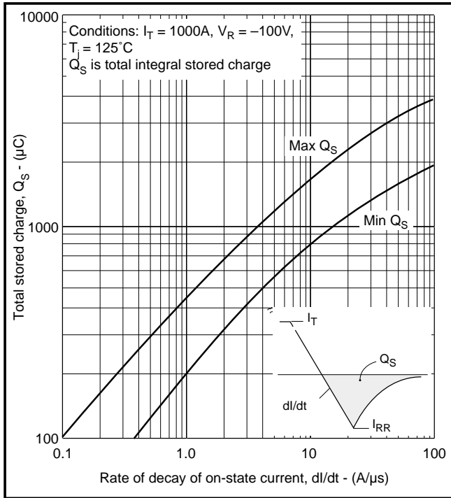
Fig.4 Stored charge
