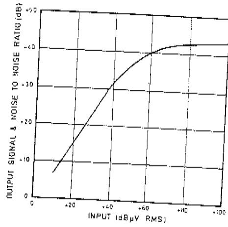
Fig. 5 Typical signal to noise ratio (S+N/NIN) with input signal (f=10.7MHz, 30% modulation)
