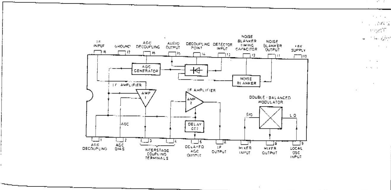
Fig. 2 SL6700C block diagram
