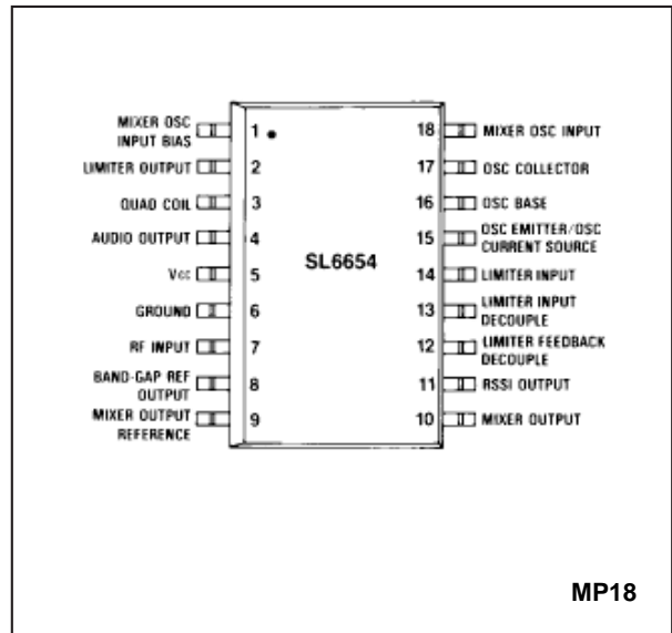
Fig. 1 Pin connections (top view)
