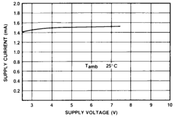
Fig. 15 Supply current vs supply voltage
