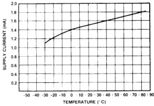
Fig. 16 Supply current vs temperature ( V_{CC} = 5V )
