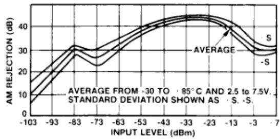
Fig. 9 AM rejection and input level
