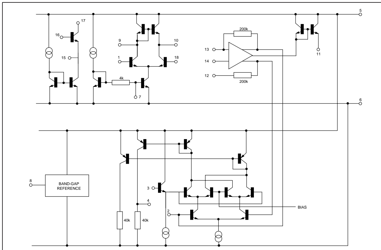
Fig. 3 Internal schematic
