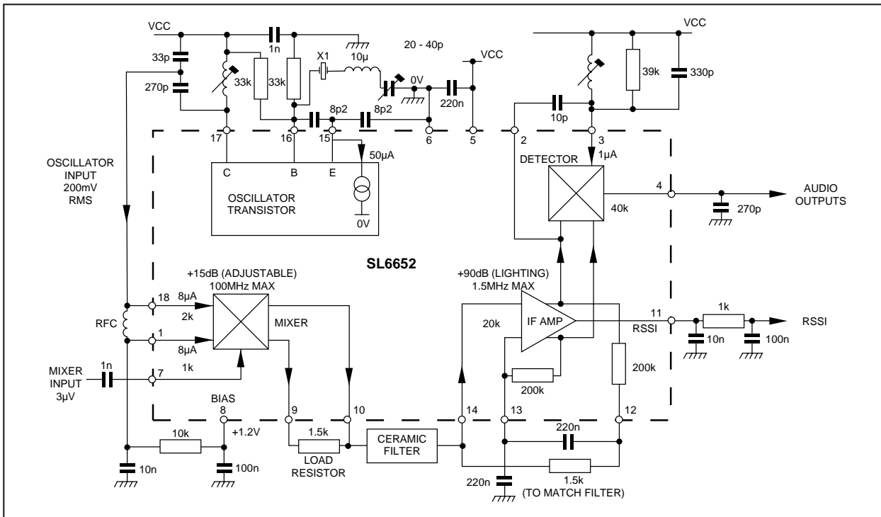
Fig. 2 block diagram
