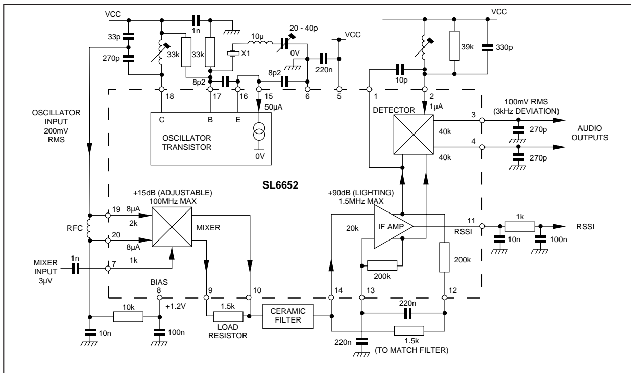
Fig. 2 block diagram
