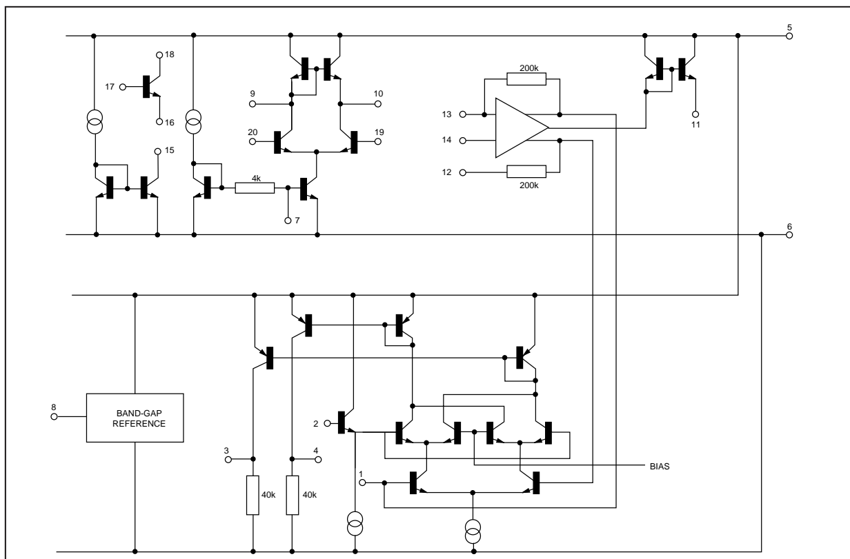
Fig. 3 Internal schematic
