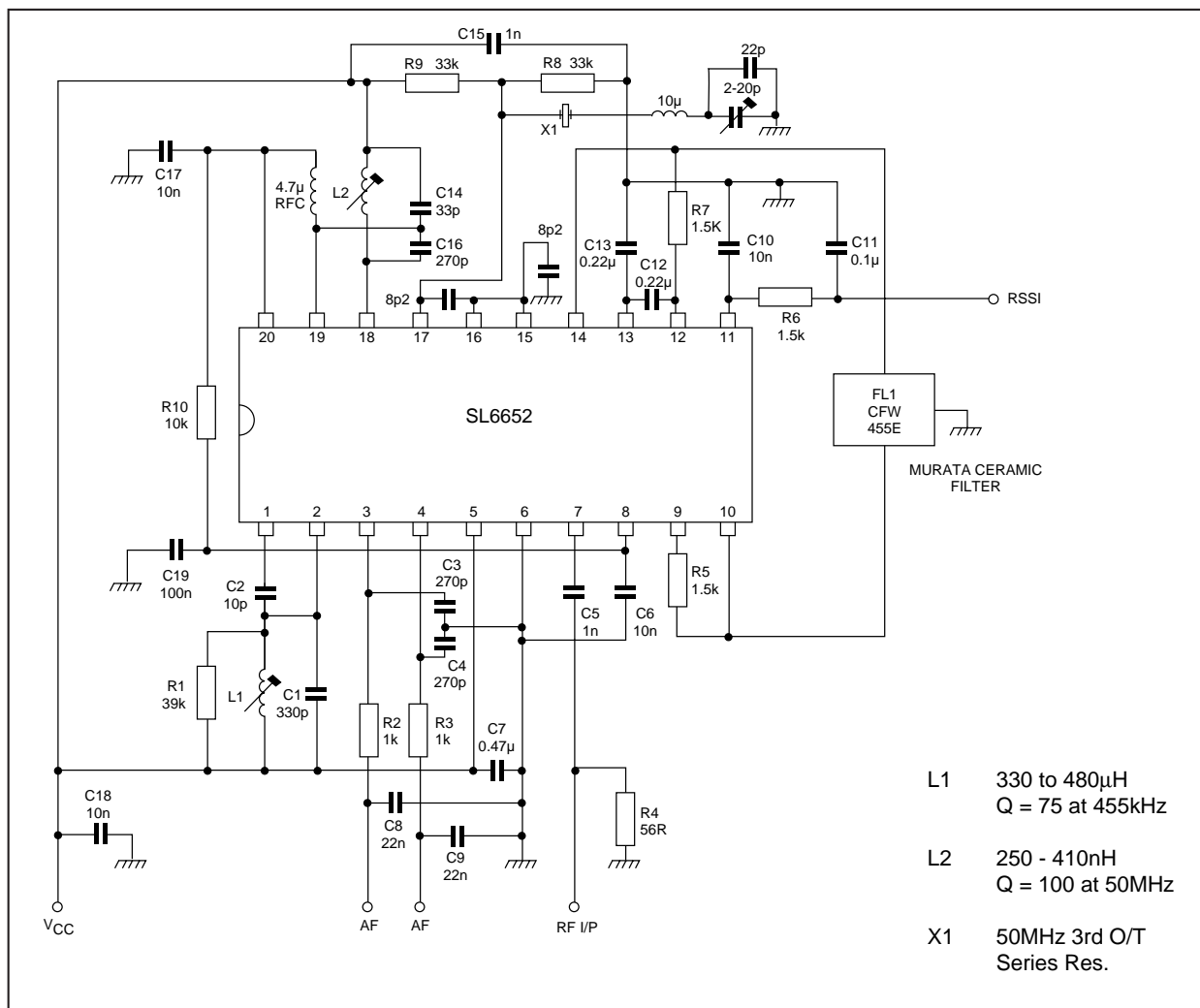
Fig. 17 Circuit diagram of SL6652 application circuit
