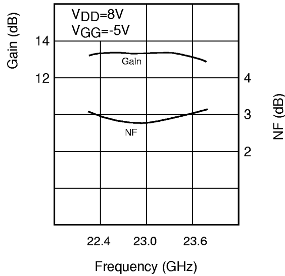
GAIN & NF vs. FREQUENCY
