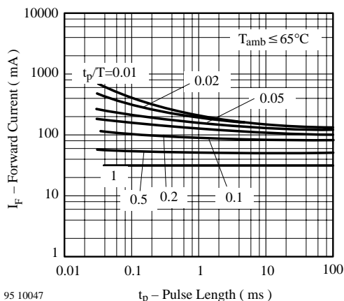
95 10047 Figure 3 Forward Current vs. Pulse Length
