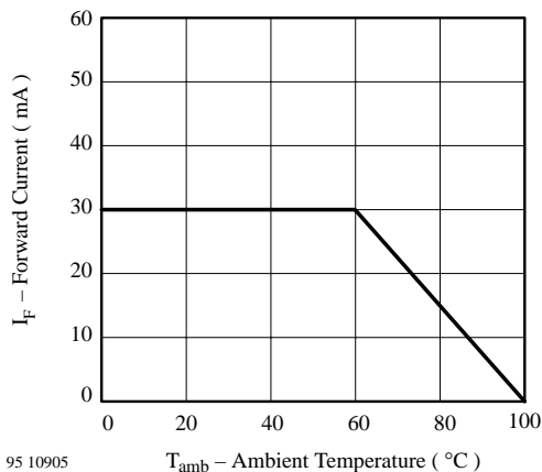
95 10905 Figure 2 Forward Current vs. Ambient Temperature
