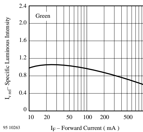
Figure 22 Specific Luminous Intensity vs. Forward Current
