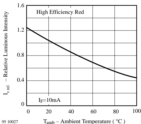
95 10027 Figure 6 Rel. Luminous Intensity vs. Ambient Temperature
