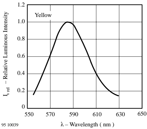
Figure 19 Relative Luminous Intensity vs. Wavelength
