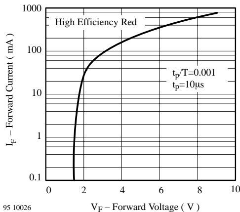
95 10026 Figure 5 Forward Current vs. Forward Voltage
