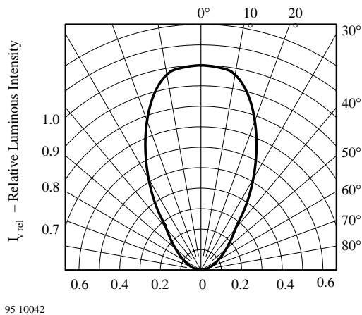
95 10042 Figure 4 Rel. Luminous Intensity vs. Angular Displacement
