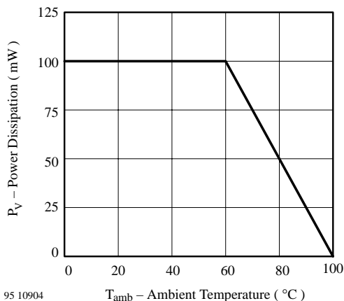
95 10904 Figure 1 Power Dissipation vs. Ambient Temperature
