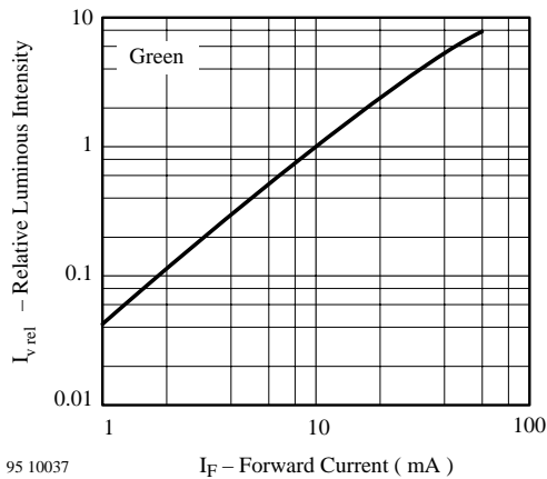
Figure 23 Relative Luminous Intensity vs. Forward Current
