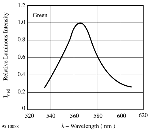
Figure 24 Relative Luminous Intensity vs. Wavelength
