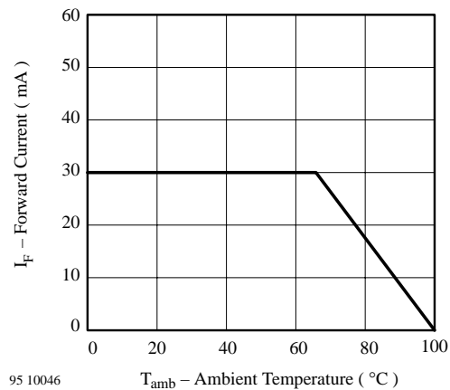
95 10046 T_{\text{amb}} – Ambient Temperature ( ^\circ\text{C} ) Figure 2 Forward Current vs. Ambient Temperature
