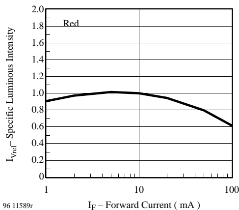
Figure 7 Specific Luminous Intensity vs. Forward Current
