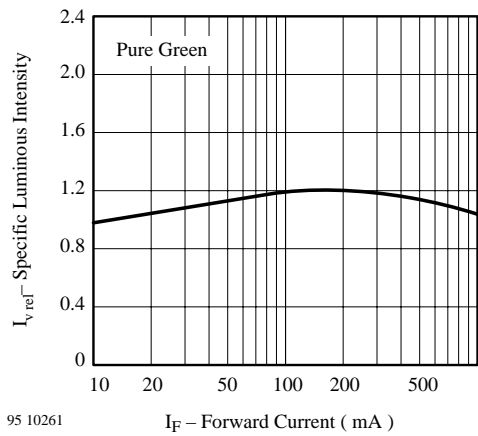
95 10261 Figure 22 Specific Luminous Intensity vs. Forward Current
