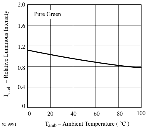
95 9991 Figure 21 Rel. Luminous Intensity vs. Ambient Temperature
