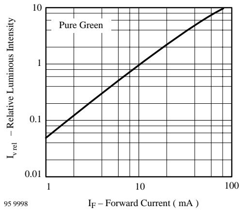
95 9998 Figure 23 Relative Luminous Intensity vs. Forward Current
