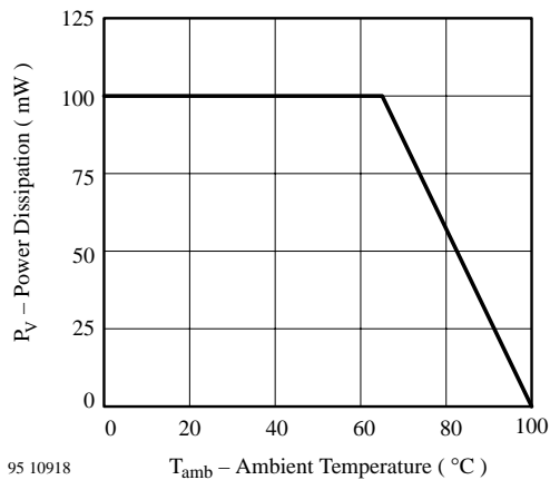
95 10918 T_{\text{amb}} – Ambient Temperature ( ^\circ\text{C} ) Figure 1 Power Dissipation vs. Ambient Temperature
