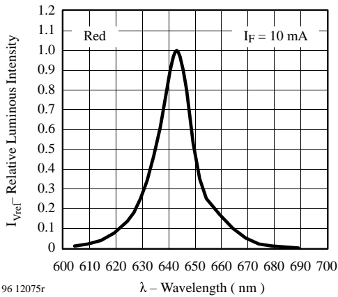
96 12075r Figure 9 Relative Luminous Intensity vs. Wavelength
