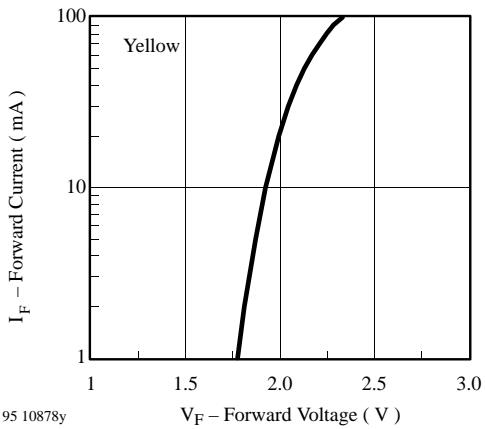
95 10878y Figure 10 Forward Current vs. Forward Voltage
