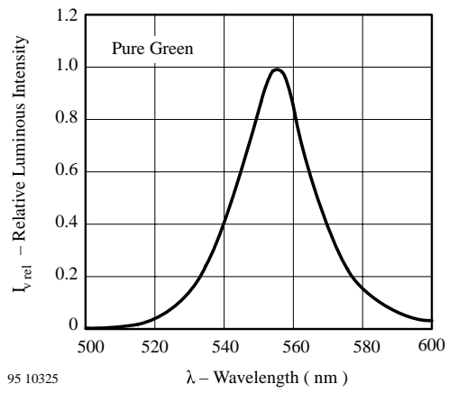
95 10325 Figure 24 Relative Luminous Intensity vs. Wavelength
