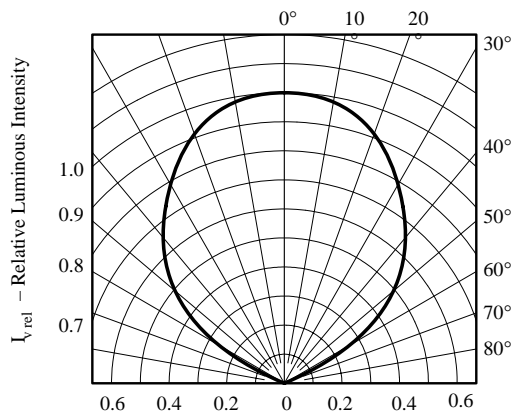
95 10082 Figure 3. Rel. Luminous Intensity vs. Angular Displacement
