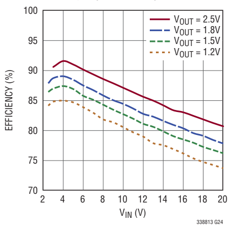
Efficiency vs V_{IN} for I_{LOAD} = 50\text{mA} , L = 22\mu\text{H} (LTC3388-1)
