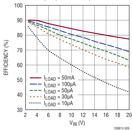
Efficiency vs V_{IN} for V_{OUT} = 1.8\text{V} , L = 22\mu\text{H} (LTC3388-1)
