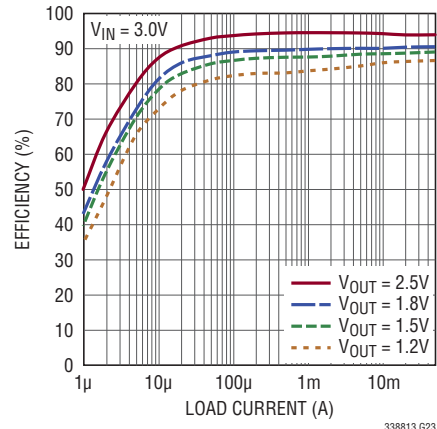
Efficiency vs I_{LOAD} , L = 100\mu\text{H} (LTC3388-1)
