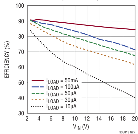
Efficiency vs V_{IN} for V_{OUT} = 1.8\text{V} , L = 100\mu\text{H} (LTC3388-1)
