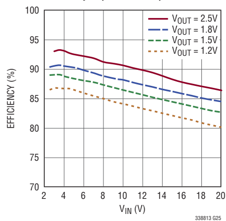
Efficiency vs V_{IN} for I_{LOAD} = 50\text{mA} , L = 100\mu\text{H} (LTC3388-1)
