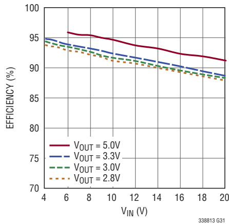
Efficiency vs V_{IN} for I_{LOAD} = 50\text{mA} , L = 100\mu\text{H} (LTC3388-3)
