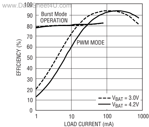
Buck-Boost Efficiency vs Load Current
