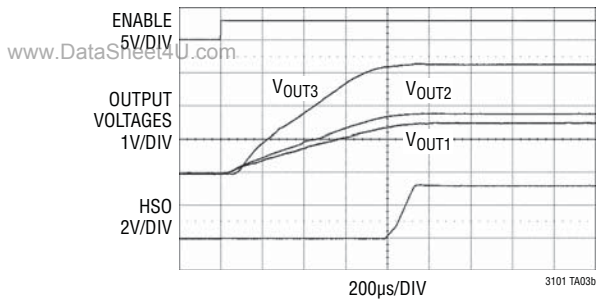
Power-Up Waveforms
