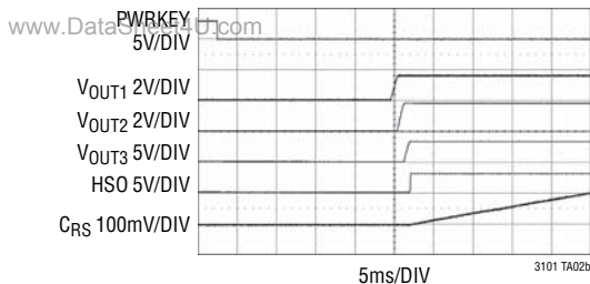
Waveforms During Power-Up
