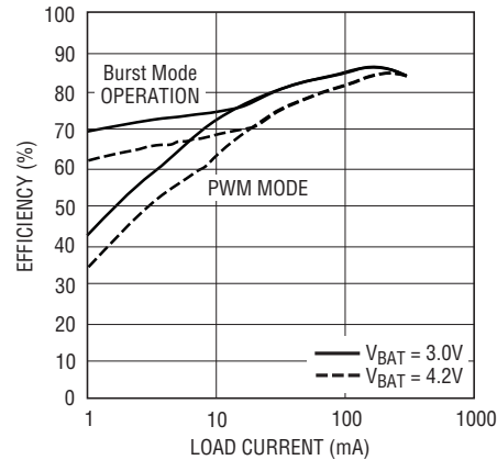
Buck Converter 2 Efficiency vs Load Current
