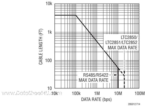
Figure 14. Cable Length vs Data Rate (RS485/RS422 Standard Shown in Solid Line)
