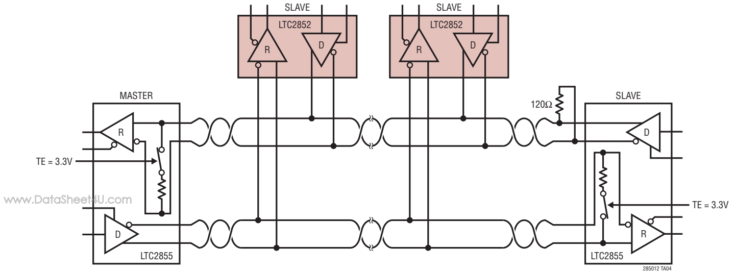
Full Duplex Network Using the LTC2852 and LTC2855
