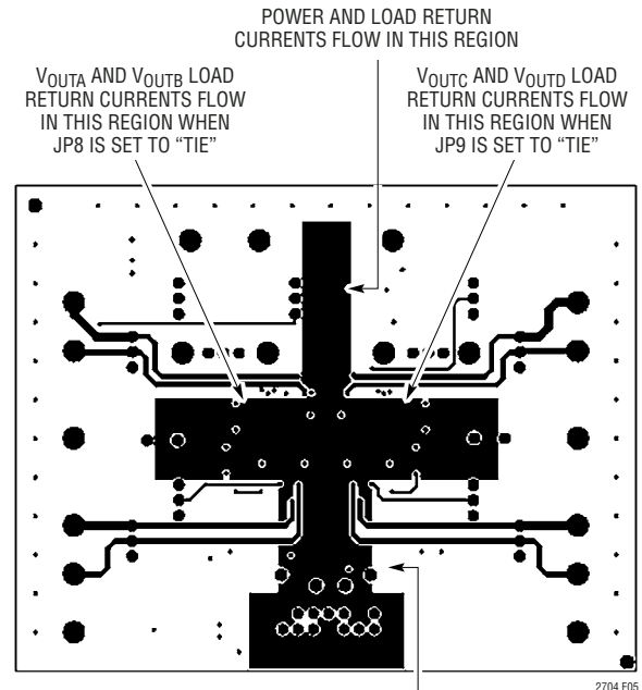
Figure 5. DC752A Load Return, Power Return and Digital Return
