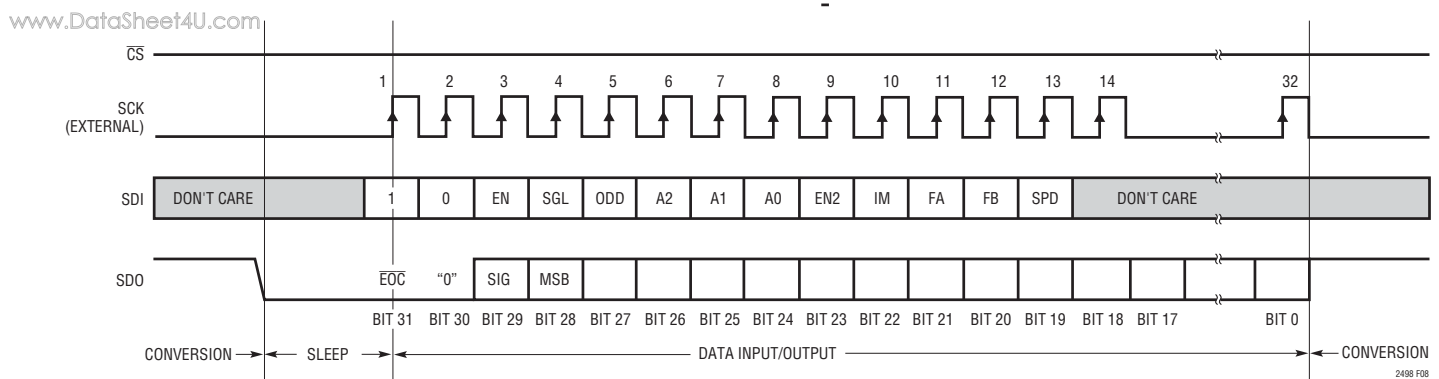
Figure 8. External Serial Clock, 3-Wire Operation ( \overline{CS} = 0 )
