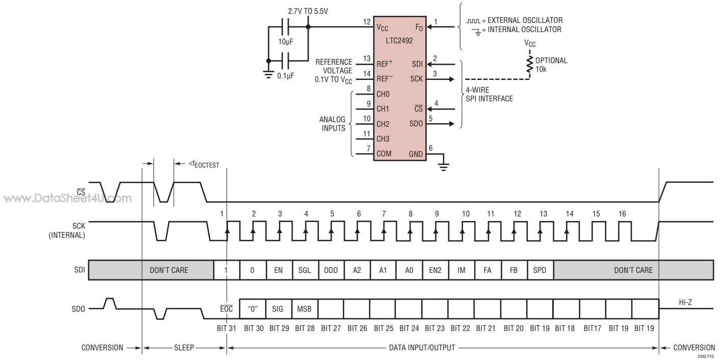
Figure 10. Internal Serial Clock, Reduced Data Output Length with Valid Channel and Configuration Selection
