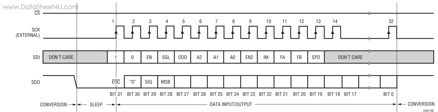
Figure 8. External Serial Clock, 3-Wire Operation ( \overline{CS} = 0 )
