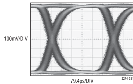
CMLOUT Eye Diagram 2.1Gbps
