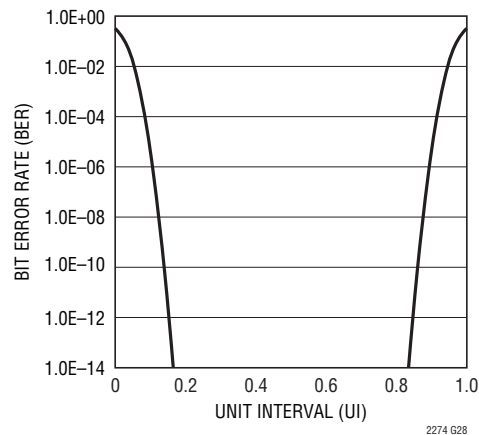
CMLOUT Dual-Dirac BER Bathtub Curve, 2.1Gbps
