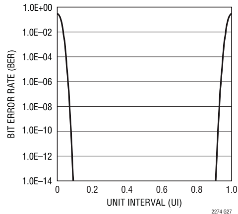
CMLOUT Dual-Dirac BER Bathtub Curve, 1.2Gbps
