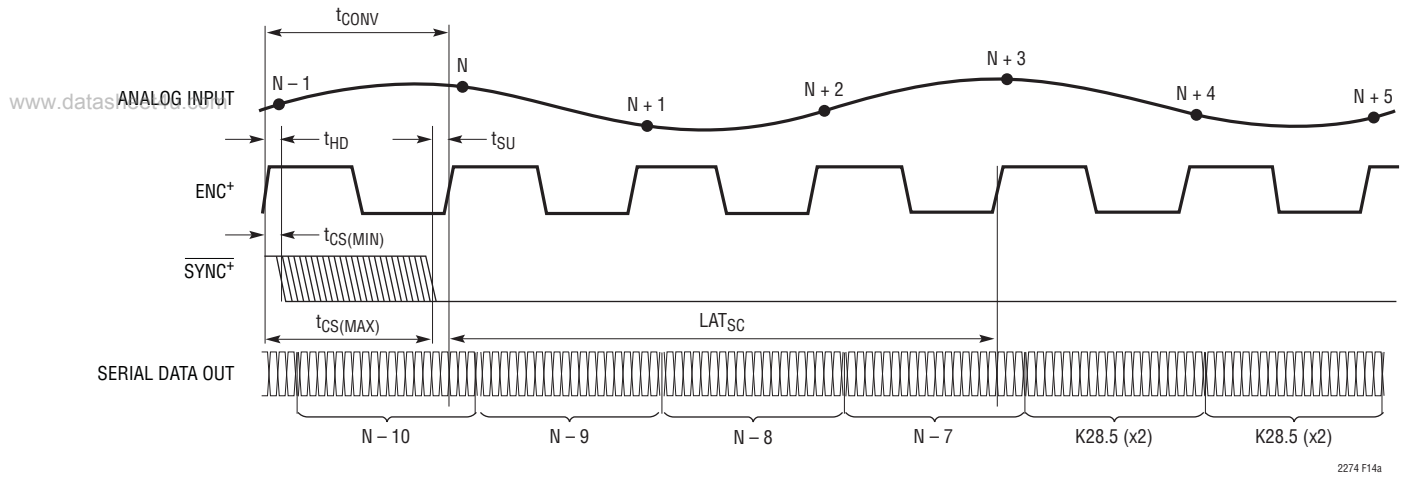
Figure 14a. \overline{\text{SYNC}}^+ Low Transition to Comma Output Timing (ISMODE is Low)
