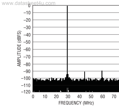
LTC2262-14: 8k Point FFT, f_{IN} = 30\text{MHz} -1dBFS, 150Mps
