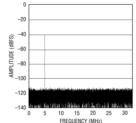
LTC2205: 64K Point FFT, f_{IN} = 5.1\text{MHz} , -40\text{dBFS} , PGA = 0, DITH = 1
