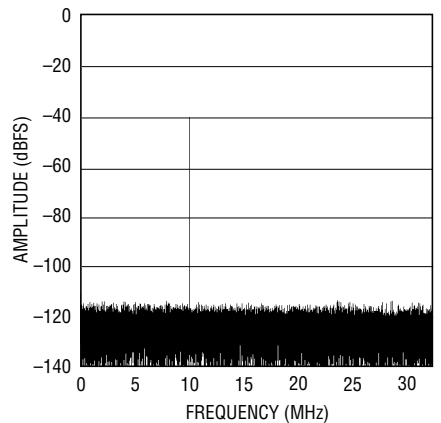
LTC2205: 64K Point FFT, 65Mps, f_{IN} = 140.1\text{MHz} , -40\text{dBFS} , PGA = 0, DITH = 1
