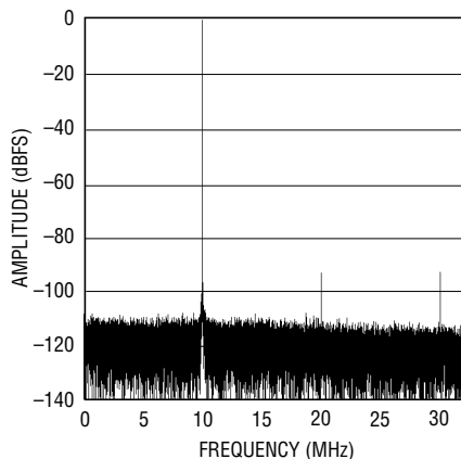
LTC2205: 64K Point FFT, 65Mps, f_{IN} = 140.1\text{MHz} , -40\text{dBFS} , PGA = 0, DITH = 0
