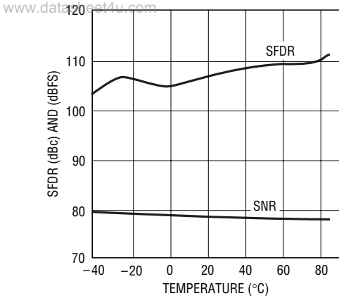
LTC2205: SFDR and SNR vs Temperature, f_{IN} = 5.1\text{MHz}
