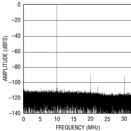
LTC2205: 64K Point FFT, 65Mps, f_{IN} = 140.1\text{MHz} , -25\text{dBFS} , PGA = 0, DITH = 1
