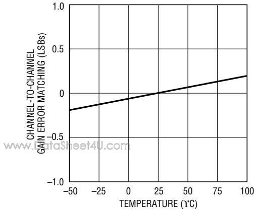
LTC1856 Channel-to-Channel Gain Error Matching vs Temperature
