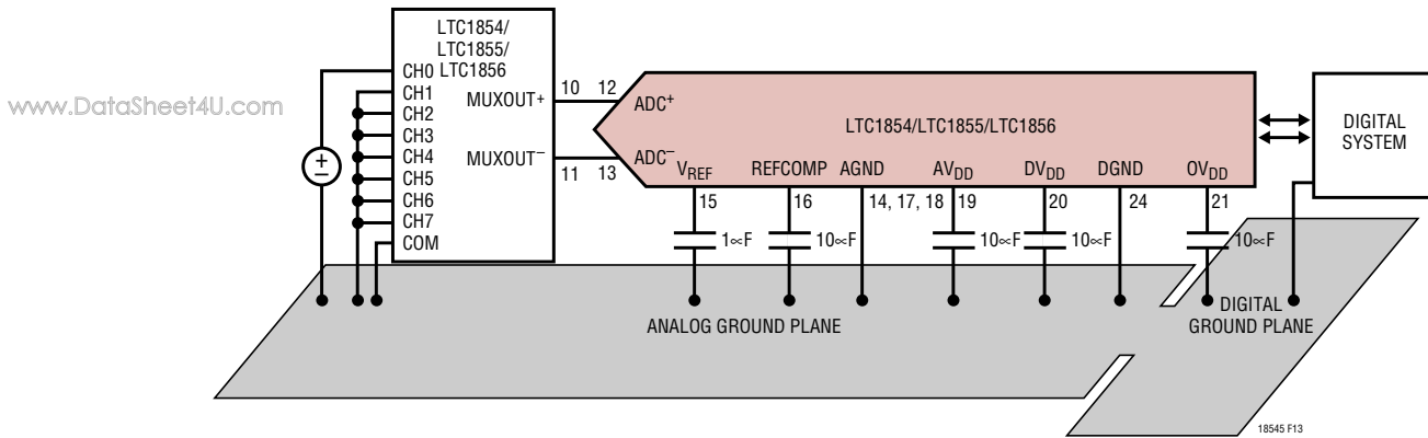
Figure 13. Power Supply Grounding Practice
