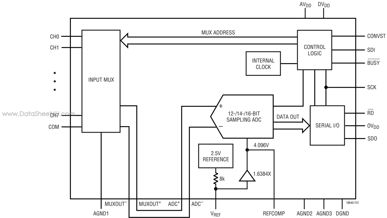
Figure 1. LTC1854/LTC1855/LTC1856 Simplified Equivalent Circuit
