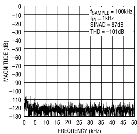
Figure 12. LTC1856 Nonaveraged 4096 Point FFT Plot
