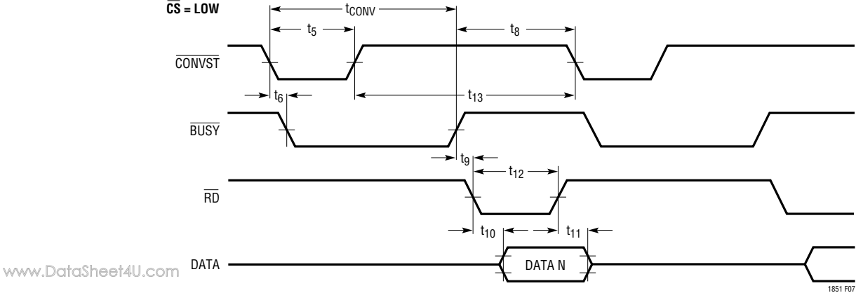
Figure 7. Mode 2 \overline{CONVST} Starts a Conversion. Data is Read by \overline{RD}
