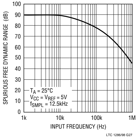
Spurious Free Dynamic Range vs Frequency
